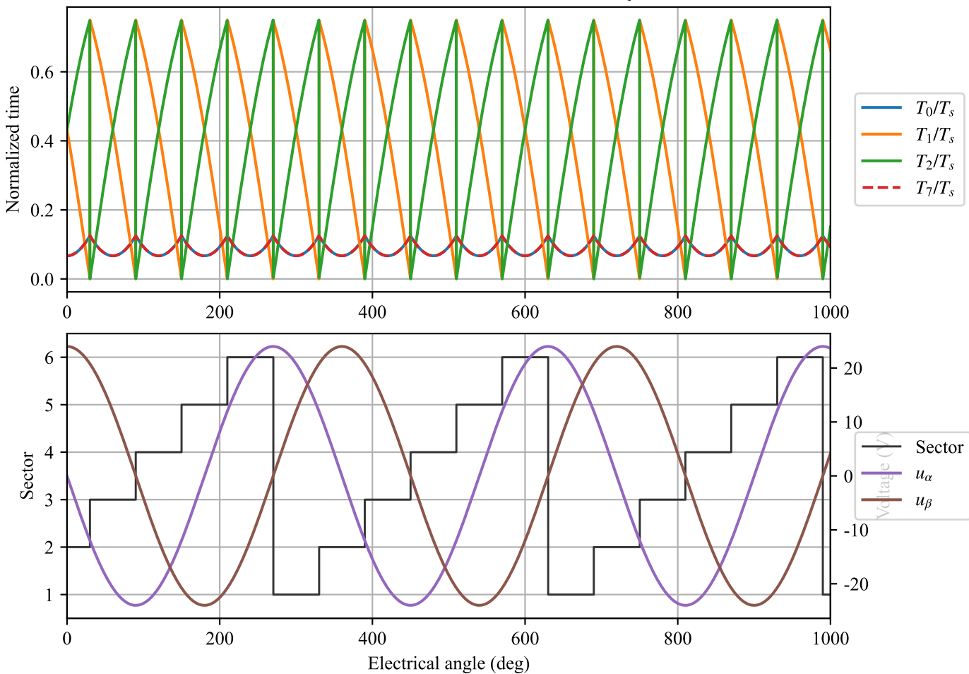
SVPWM timing curves, U_{dc}=48\text{ V} , u_d=0\text{ V} , u_q=24\text{ V}
